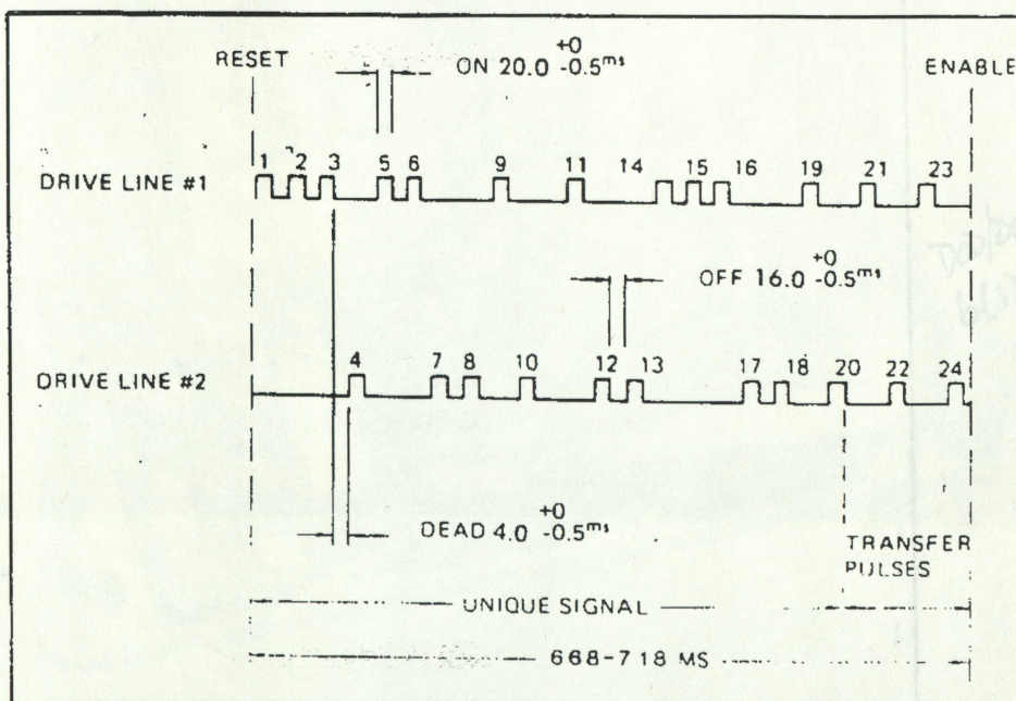
Figure 10. Trajectory Unique Signal (TUQS)
